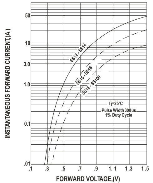
FIG.2-TYPICAL FORWARD CHARACTERISTICS
